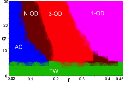
Fig. 3: Map of dynamic regimes for N = 100 in the plane of coupling strength \sigma and coupling range r . 1-OD: one-cluster oscillation death; 3-OD: three-cluster oscillation death; N-OD: multi-cluster ( > 3 ) oscillation death; AC: amplitude chimera; TW: traveling wave. Other parameters: \lambda = 1 , \omega = 2 .
