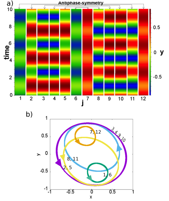
Fig. 8: (a) Space-time plot of an amplitude chimera state y_j(t) in a very small network. (b) Phase portrait. Parameters: N = 12 , \lambda = 1 , \omega = 2 , r = \frac{1}{12} , \sigma = 5 .
