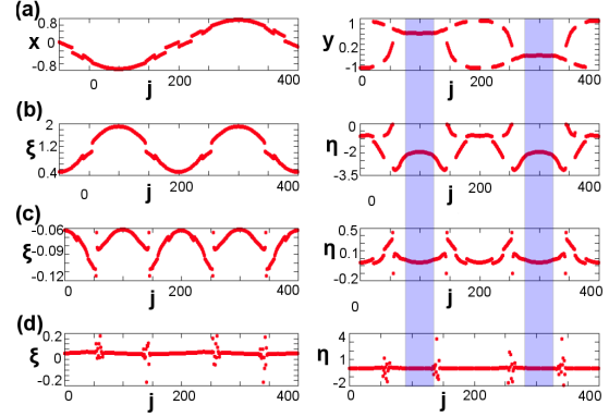
Fig. 6: Real (left column) and imaginary parts (right column) of (a) snapshot z_j , (b) eigenvectors associated with the largest positive \Lambda = 0.135 , (c) with the second positive \Lambda = 0.053 , (d) with the first negative \Lambda = -0.133 . Shaded regions mark the coherent domains. Parameters: N=400 , \lambda = 1 , \omega = 2 , \sigma=23 , r=0.06 .
