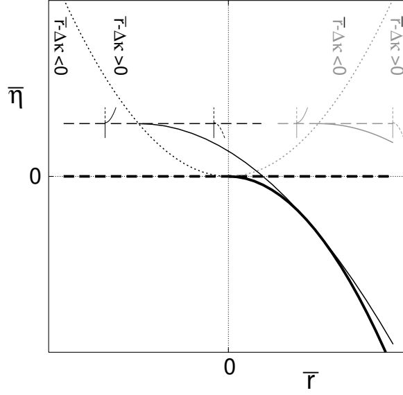
Figure 2. Sketch of a partial bifurcation diagram of the amplitude equation (2) in the \bar{r} - \bar{\eta} plane. The thick broken line indicates the instability of the trivial state. The thin broken line represents the bifurcation of plane waves from the trivial state for a wave number \kappa with \Delta\kappa > 0 (cf. eq.(45)). The pitchfork like inserts indicate whether the bifurcations are sub- or supercritical and the thin dotted line gives the transition for all wavenumbers (cf. eq.(47)). The thin solid line marks the saddle node bifurcation for the plane wave (cf. eq.(49)). The corresponding features for the wavenumber -\kappa are displayed in grey. Finally the thick solid line marks the envelope of saddle node bifurcation lines for all wavenumbers (cf. eq.(51)).
