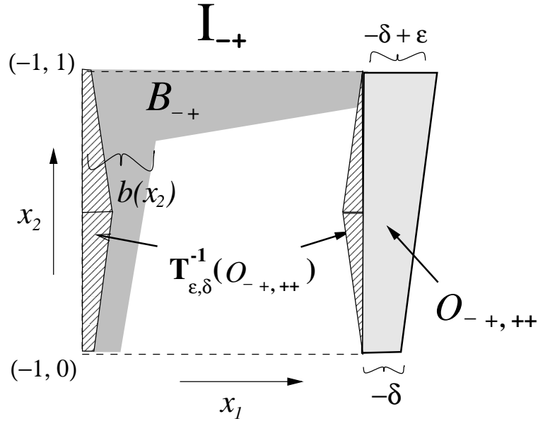
FIG. 5. Overlap set O_{-+,++} and its pre-image set \mathbf{T}_{\epsilon,\delta}^{-1}(O_{-+,++}) are shown for \delta = -\epsilon . The forbidden area B_{-+} \subset I_{-+} contains the pre-images of O_{-+,++} on the left side.
