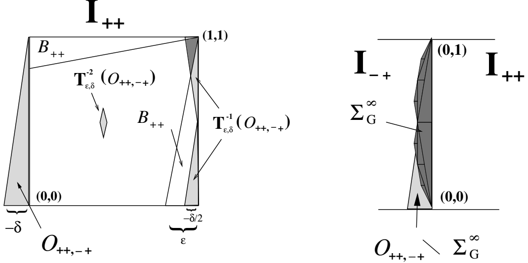
FIG. 8. Left: Overlap set O_{++,-+} and pre-image sets of first and second generation are shown. Note that the dark shaded subset of \mathbf{T}_{\epsilon,\delta}^{-1}(O_{++,-+}) is located outside the forbidden area B_{++} . Right: The overlap set O_{++,-+} intersects the set \Sigma_G^\infty (approximated here by three pre-image generations).
