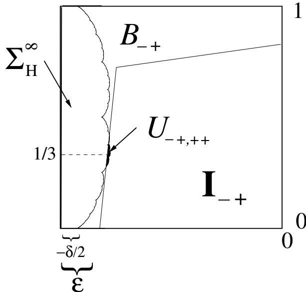
FIG. 7. Non-empty transition set U_{-+,++} := \Sigma_H^\infty \setminus B_{-+} for \delta slightly smaller than \delta_{crit}(\epsilon) . The set \Sigma_H^\infty is no longer contained in the forbidden area B_{-+} for these \delta values.
