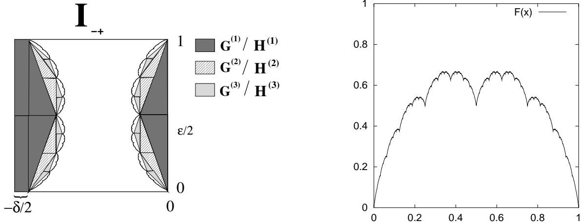
FIG. 6. Left: The first three generations G^{(k)} and H^{(k)} near the right and left edge of I_{-+} , respectively. The envelopes R^\infty and S^\infty of all pre-image sets G^{(k)} and H^{(k)} , respectively, are related to the Takagi function. Right: Takagi function F(x) .
