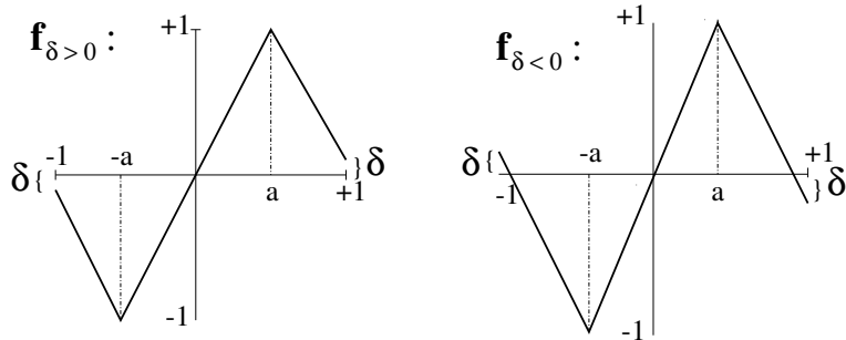
FIG. 1. The deformed antisymmetric tent map f_\delta .
