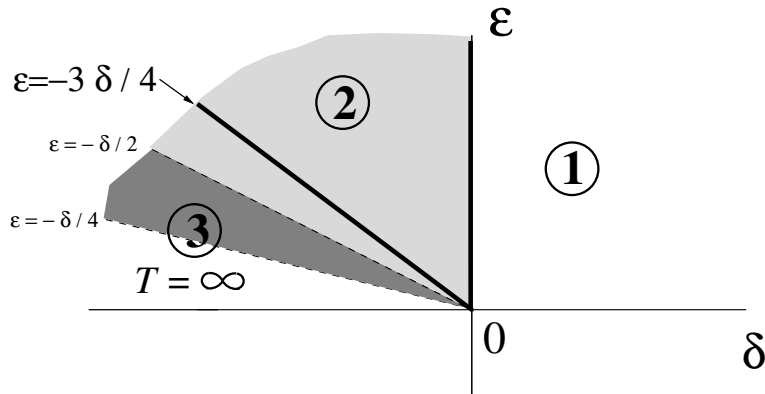
FIG. 2. Diagrammatic view of the bifurcation diagram for the unidirectional CML \mathbf{T}_{\epsilon,\delta} . The three parameter regions of section V are labeled by numbers. Gray shading indicates the type of coupling in the corresponding kinetic Ising model, antiferromagnetic (light) or ferromagnetic (dark). There is also a region where the temperature is \infty .
