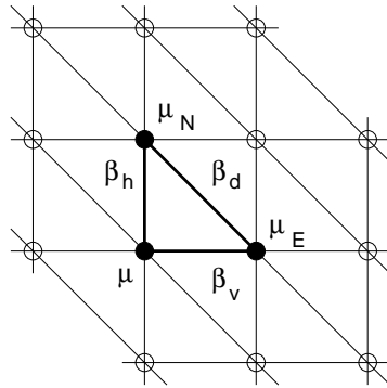
Fig. 1 Coupling scheme of the Hamiltonian (10) which determines the stationary density of the Toom-Glauber model.
