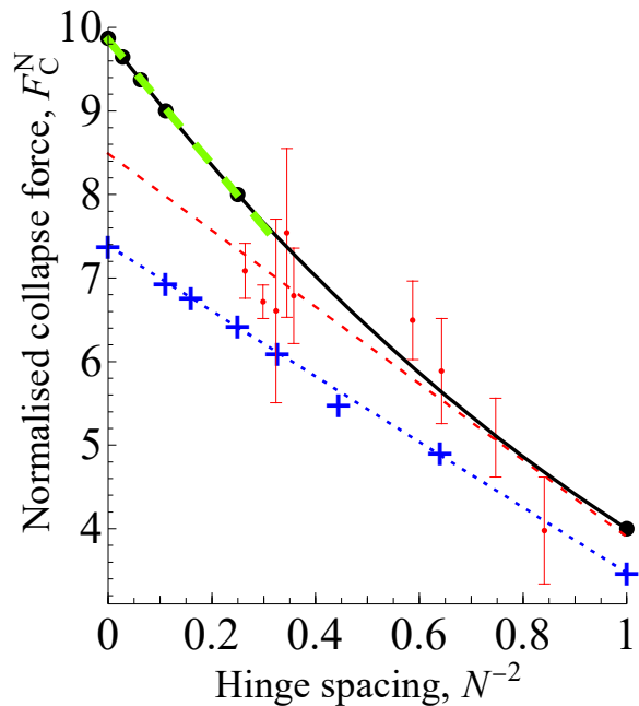
FIG. 3. The normalized collapse force F_C^N of Eq. (2) is plotted against N^{-2} where N is the number of hinges per half-wavelength of a buckling mode of an infinite chain with k = \pi (solid black line), or, equivalently, the number of hinges in a column of unity length. Results from calculations for integer N are plotted (solid circles), for N = 1 - 4, 6, \infty . The green dashed line is the least-squares fit of Eq.(3) to these data excluding N = 1 . The blue crosses are the numerical data for the collapse of m -gons [12], plotted for m = 4 - 8, 10, 12, \infty . This data is rescaled by converting pressure to circumferential force, and using m = 4N . The blue dotted line is the least-squares fit to these data. The experimental data for nanotubes [10] are shown by red datapoints with error bars and fitted by the red dashed line, scaled to these axes as described in the text.
