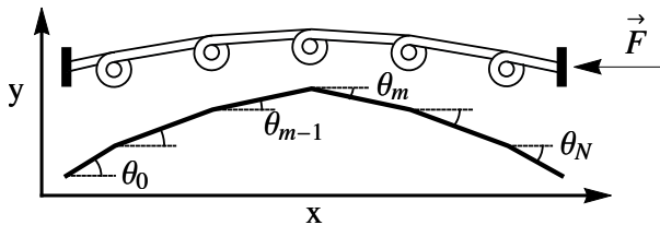
FIG. 2. A pillar along the x -axis is discretized to have compliance only at N angular hinges of stiffness c . The lower part of the graph shows a chain of rigid rods numbered \mu = 0 to N at angles \theta_\mu . Buckling causes y -axis displacements of the hinges y_\mu ( \mu = 1 to N ).
