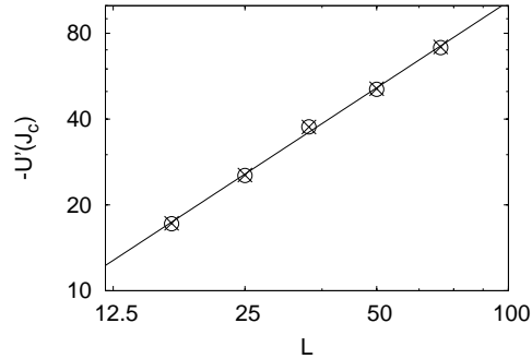
FIG. 7: Derivative of the Binder cumulant at the critical coupling strength in dependence of the system size. Data points have been obtained from the cubic ( \times ) and quartic ( \circ ) fit to the data displayed in figure 6. The straight line shows a least square fit.
