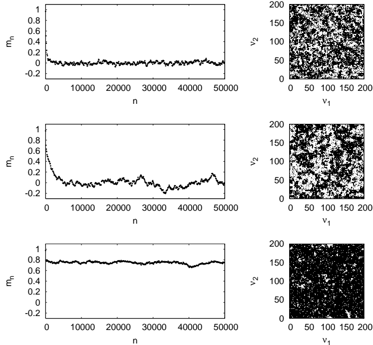
FIG. 5: Numerical simulation of the coupled map lattice (21), (23) for J_0 = 1.25 on a square lattice of size 200 \times 200 with periodic boundary conditions. Time dependence of the magnetisation m_n = \sum_{\nu} \sigma_n^{(\nu)} / L^2 (left) and final state of the symbol lattice at n = 50000 (right) when a ferromagnetic initial state has been used. Top: subcritical coupling J_{nn} = 0.20 , middle: "critical" coupling J_{nn} = 0.22 , bottom: supercritical coupling J_{nn} = 0.24 .
