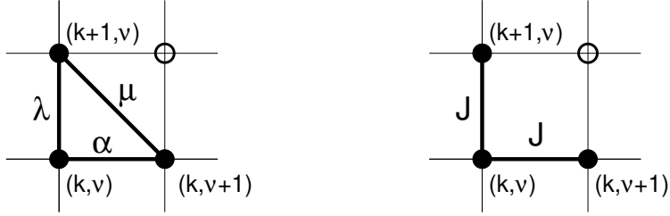
FIG. 3: Diagrammatic view of the interactions in the two-dimensional Ising Hamiltonians eq.(18) (left) and eq.(20) (right).
