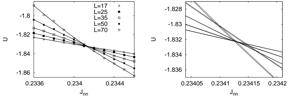
FIG. 6: Left: Numerical computation of the Binder cumulant (28) for the coupled map lattice (21), (23) with J_0 = 1.25 and different system sizes. For each value of the system size L the lines display a cubic and quartic least square fit to the data points. The two lines cannot be distinguished at the scale of the graph. Right: Graph of the Binder cumulants on a smaller scale. Cubic and quartic fits to the data points can now be distinguished.
