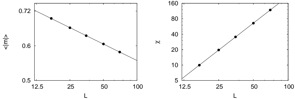
FIG. 8: Left: Dependence of the first moment of m = \sum_{\nu} \sigma^{(\nu)} / L^2 at J_c = 0.23413 on the system size L . The straight line shows a least square fit with slope = -0.1245 \pm 0.0005 . Right: Dependence of the finite size susceptibility (31) at J_c on the system size L . The straight line indicates a least square fit with slope 1.748 \pm 0.003 .
