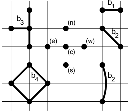
FIG. 10: Labelling of the "central" lattice site (c) and its four nearest neighbours (e), (n), (w), and (s). Diagrammatic view of the two spin and four spin interactions appearing in the local energy contribution (C2), apart from rotations.
