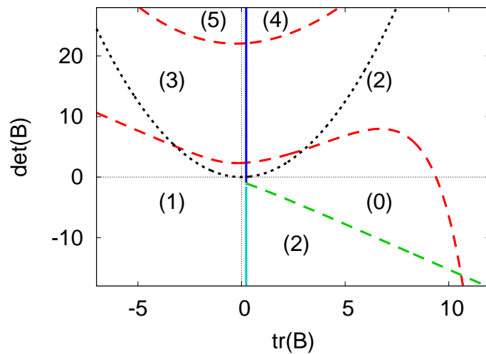
FIG. 9: (Color online) Bifurcation diagram of the characteristic equation (B2) in a two-dimensional parameter plane for \gamma = -10 , \beta = \pi/4 , and \lambda = -0.02 . Solid blue/cyan: transcritical bifurcation, Eq. (B6) (unstable eigenvalue occurs left/right of the line). Dashed red/green: Hopf bifurcation, Eq. (B8) (unstable eigenvalues occur above/below the line). Dotted black: bifurcation path traced by the control scheme, cf. Eq. (B10). Labels indicate the number of unstable eigenvalues.
