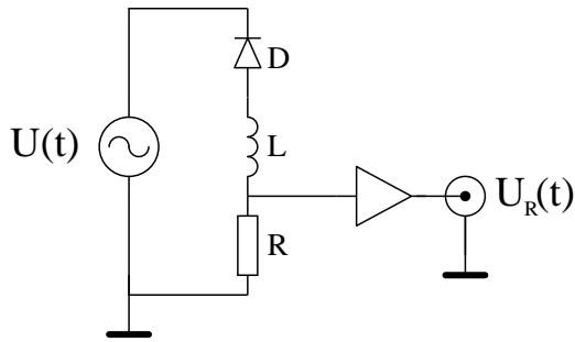
FIG. 1: Diode resonator circuit consisting of a 1N4006 diode, an inductor L = 1\text{mH} , a resistor R = 51\Omega , and a sinusoidal drive U(t) = U_0 \sin(\Omega t) with amplitude U_0 = 0\text{V} \dots 6\text{V} and frequency \Omega/2\pi = 1\text{MHz} . Additional components for shielding and extracting the signal which were implemented to minimise noise and cross-talk are not shown.
