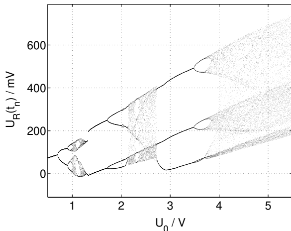
FIG. 2: Bifurcation diagram of the diode resonator constructed from the maxima of the output signal U_R(t) at discrete times t_n .
