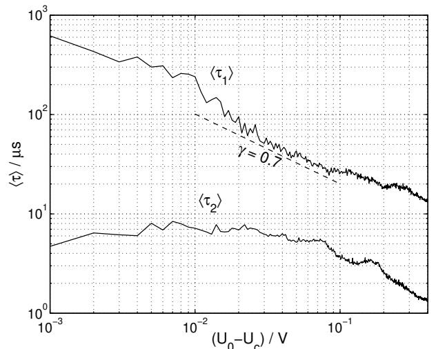
FIG. 8: Mean residence times of the diode resonator evaluated from the symbolic time series. \langle \tau_1 \rangle follows a power law with a scaling exponent \gamma of 0.7 as predicted in [20].
