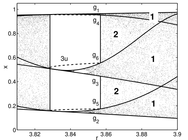
FIG. 5: Skeleton of the logistic map in a neighbourhood of the period three window. Solid lines: first six iterates g_n(r) of the critical point; broken line: unstable period-three orbit. Labels refer to the phases 'Ch1' and 'Ch2'.
