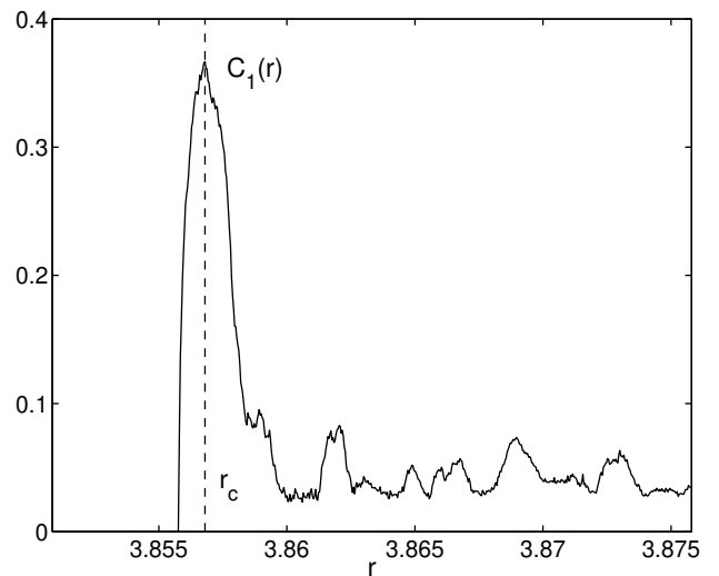
FIG. 10: Noise-free stochastic resonance of the logistic map. Normalised cross correlation function C_1 between the output signal \sigma_n and the modulation \tilde{r}_n . The period of the modulation signal is T_m = 100 iteration steps, which is comparable to the parameters \omega/\omega_m chosen for the diode resonator.
