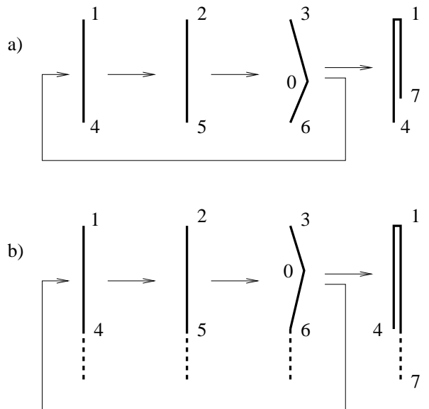
FIG. 7: Diagrammatic view of the folding and stretching process of a chaotic three-band attractor. a) Below the crisis. Labels refer to the images of the 'critical point' g_0 , solid lines visualise the three bands which are mapped onto each other. b) Beyond the crisis. Dashed lines indicate those parts which are not mapped onto each other any more.
