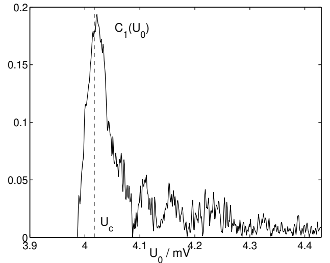
FIG. 9: Noise-free stochastic resonance of the diode resonator evaluated in terms of the normalised cross correlation function between the symbolic time series and the modulation signal, eq.(5).
