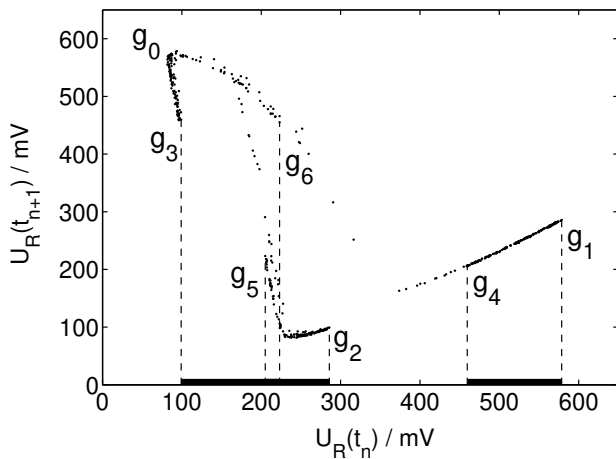
FIG. 6: Return map constructed from the local maxima of the experimental time series U_R(t) close to the crisis. Labels refer to the critical point and its images. The rightmost branch of the 'Ch1'-phase remains well separated, while the other branches overlap with each other and with parts of the 'Ch2'-phase.
