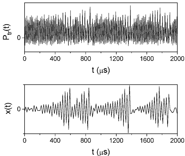
FIG. 11. Example of a time series showing type-III intermittency. \nu = 2.385 GHz, H = 800 Oe, P_{in} = 8.49 dBm. Top: Original signal; the laminar intervals exhibit the typical spreading up of successive maxima. Bottom: Same signal averaged over one period.
