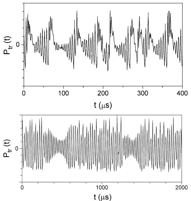
FIG. 3. Examples of time series showing type-I intermittency. Top: \nu = 2.414 GHz, H = 840 Oe, P_{in} = 0.66 dBm. Lamellar intervals are characterized by increasing oscillation amplitudes and interrupted by short chaotic bursts. Bottom: \nu = 2.496 GHz, H = 840 Oe, P_{in} = 7.04 dBm. The lamellar intervals correspond to ‘channels’ of small-amplitude oscillations separated by large-amplitude chaotic intervals of long duration.
