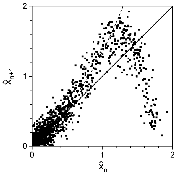
FIG. 12. First-return map extracted from the time series of Fig. 11 (bottom). The dashed line is a fit to the second iterate of eq.(4) generic for type-III intermittency: x_{n+2} = 1.056x_n + 0.291x_n^3 . In order to exclude the reinjecting part of the map, our fit was restricted to x_n \leq 1.2 .
