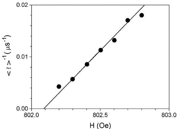
FIG. 19. Dependence of the inverse mean 'laminar' length on magnetic field. The straight line fitted to the data corresponds to the scaling exponent -1 and yields the bifurcation point H_c = 802.09 Oe.
