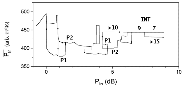
FIG. 2. Multistability in the coincidence regime ( \nu = 2.37 GHz, H = 840 Oe). The averaged transmitted power \overline{P_{tr}} is plotted vs. the input power P_{in} (normalized to the Suhl threshold). Different dc-levels correspond to different types of dynamics. Periodic behaviour is indicated by its periodicity (P1, P2), and chaotic behaviour by the attractor dimension (accuracy \pm 1 ). Chaos-chaos intermittency is observed at the upper chaotic level (INT).
