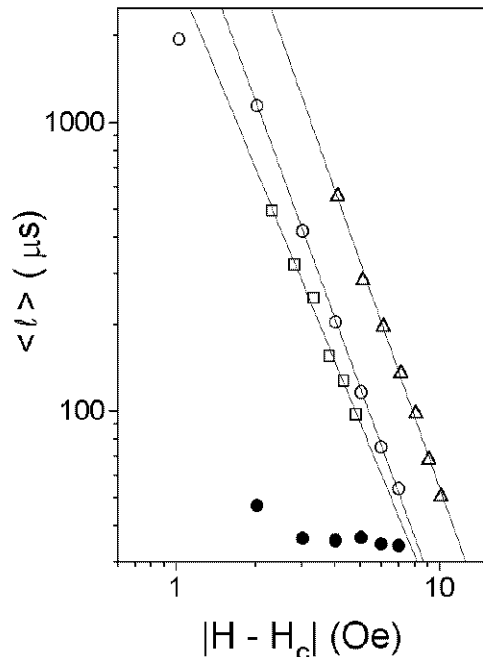
FIG. 16. Scaling behaviour of the mean 'laminar' length with respect to the magnetic field. Data were taken at three different microwave powers: 15.5 dB ( \square ), 16.5 dB ( \circ ), 17.0 dB ( \triangle ). The double-logarithmic plot yields scaling exponents \gamma = 2.2, 2.5 , and 2.6 , respectively. Bullets denote mean length of the bursts for P_{in} = 16.5 dB, which is nearly field independent.
