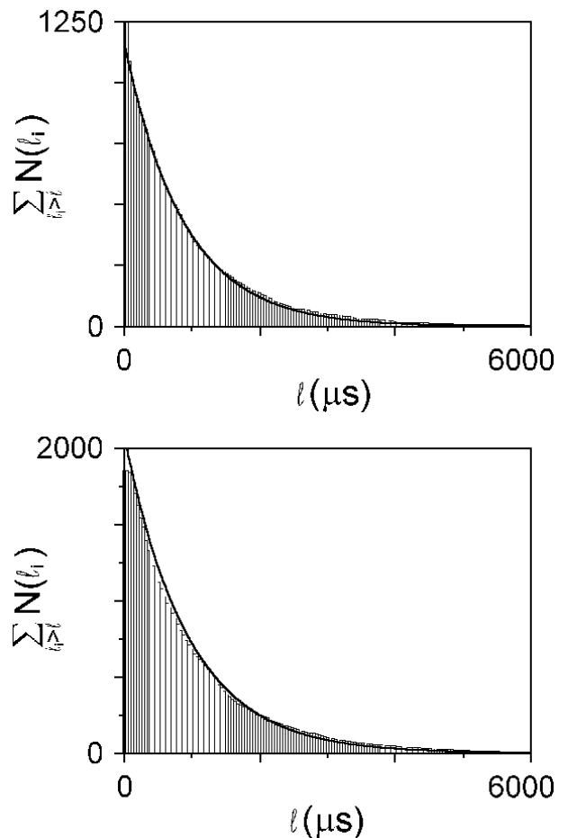
FIG. 21. Integrated distribution of the laminar (top) and chaotic (bottom) lengths for the time series shown in Fig. 20. The solid lines are fits to an exponential distribution expected for noise-induced intermittency.
