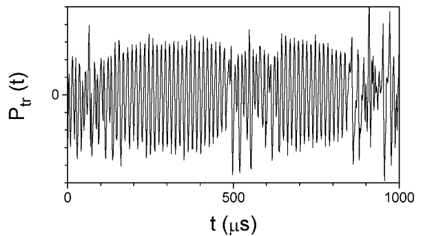
FIG. 20. Intermittent time series measured in the coincidence regime ( \nu = 2.3887 GHz, H = 840 Oe, P_{in} = 7 dBm).
