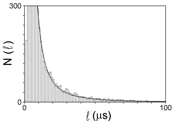
FIG. 9. Experimental distribution of the laminar lengths. \nu = 9.255 GHz, H = 1592 Oe, P_{in} = 15.5 dB. The solid line is a fit to the theoretical distribution for type-II intermittency, eq. (3).
