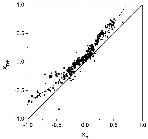
FIG. 4. First-return map extracted from the time series of Fig. 3 (bottom). The dashed line is a fit to the quadratic map, eq.(2), generic for type-I intermittency: x_{n+1} = 0.092 + 1.045x_n + 0.273x_n^2 .
