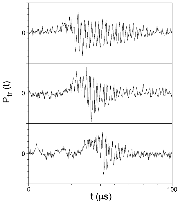
FIG. 15. Extended plot of the chaotic bursts. The input microwave power P_{in} amounts to (from top to bottom): 15.5 dB, 16.5 dB, 17.0 dB.
