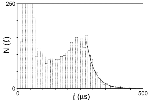
FIG. 6. Experimental distribution of laminar lengths of the time series shown in Fig. 3. Data set consisted of 7.5 \cdot 10^5 data points. The solid line is a fit to the exponential tail of the distribution.
