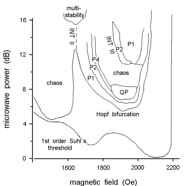
FIG. 1. Dynamics in the subsidiary absorption regime ( \nu = 9.26\text{GHz} ) with respect to magnetic field H and input microwave power P_{in} . The lowest line indicates the Suhl threshold, the lines above separate regimes of different time behaviour, e.g. period doublings (P2, P4), quasiperiodicity (QP), or chaos. Intermittency is observed in several parameter regimes, e.g. type II at 1650 Oe / 12-15 dB; type III at 1900 Oe / 11-15dB; crisis-induced intermittency at 1900 Oe / 16 dB.
