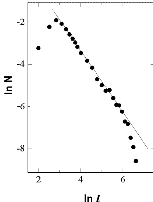
FIG. 18. Distribution of the 'laminar' lengths, i.e. the time intervals between two bursts, from the time series shown in Fig. 17. \ell is measured in \mu s . The solid line corresponds to a power-law scaling of -3/2 .
