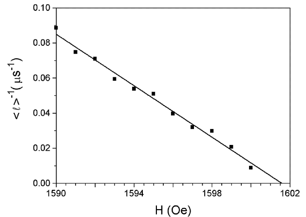
FIG. 10. Inverse mean laminar length \langle l \rangle^{-1} vs. magnetic field H . The solid line represents a least square fit to a linear dependence and yields H_c = 1601.5 Oe.
