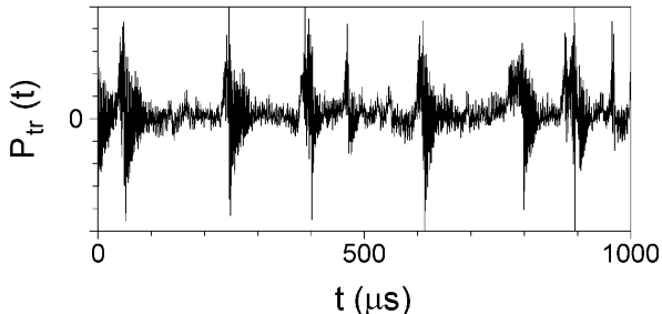
FIG. 14. Time series representing a homoclinic crisis at \nu = 9.258 GHz, H = 1877 Oe, P_{in} = 16.5 dB (cf. Fig. 1).
