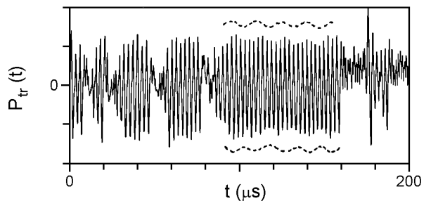
FIG. 7. Example of a time series showing type-II intermittency. \nu = 9.257 GHz, H = 1590 Oe, P_{in} = 15 dB. The laminar intervals are quasiperiodic, the low-frequency amplitude modulation has been stressed by the dashed envelopes.
