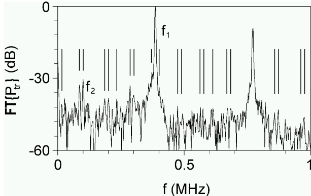
FIG. 8. Fourier spectrum of the time series shown in Fig. 7. Two fundamental frequencies occur at f_1 = 385 kHz and f_2 = 100 kHz. All strongest spectral components, indicated by vertical bars, were identified to present mixing frequencies m \cdot f_1 + n \cdot f_2 , m, n integer, |m| \leq 3 and |n| \leq 10 . The frequency splitting \Delta = 4f_2 - f_1 = 15 kHz occurring everywhere in the spectrum reflects the amplitude modulation of the time series.
