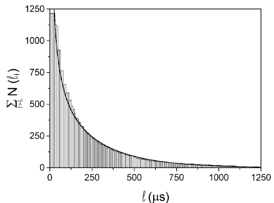
FIG. 13. Integrated experimental distribution of the laminar lengths. The solid line is a fit to the theoretical distribution for type-III intermittency.
