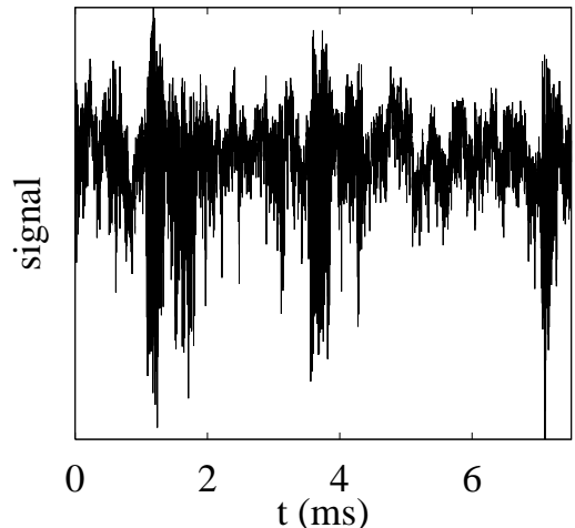
FIG. 17. Time series showing on-off intermittency in the coincidence regime ( \nu = 2.388 GHz, H = 802.5 Oe, P_{in} = 14.5 dBm).
