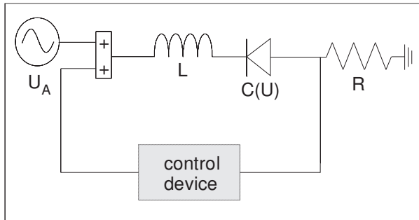
FIG. 8. Experimental setup of the nonlinear diode resonator with control device.
