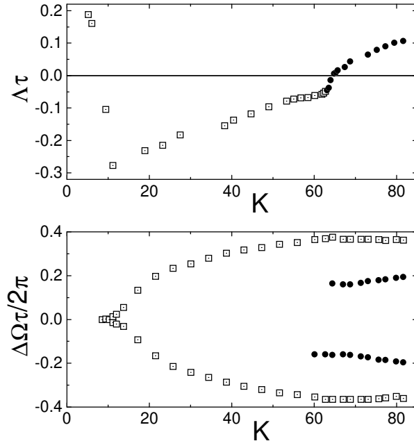
FIG. 13. Floquet branch with largest real part and frequency deviation for the period-one orbit of the nonlinear diode resonator in dependence on the control amplitude: open symbols – branch connecting to the free unstable Lyapunov exponent, full symbols – crossing complex branch.
