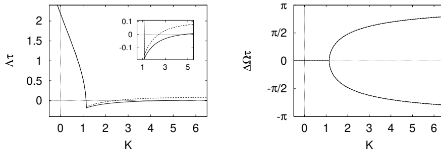
FIG. 3. Real part of the largest Floquet exponent and frequency deviation for the period-four orbit of the Toda model (12) in dependence on the control amplitude (solid lines). The inset shows an enlargement of the control interval. Dotted lines display results according to the analytical expressions (13) and (6), but partly hidden since the coincidence is almost within the resolution of the figure.
