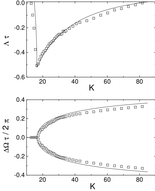
FIG. 10. Floquet branch with largest real part for the period-one orbit of the nonlinear diode resonator in dependence on the control amplitude. Solid lines display fits according to the analytical result (8) with \lambda\tau = 1.07 and (-\tau\chi_R) = 0.036 .
