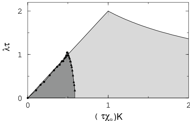
FIG. 12. Control domain for the diode resonator in the plane of control amplitude and free Lyapunov exponent: circles – lower threshold (flip bifurcation), triangles – upper threshold (Hopf bifurcation). Solid line and light gray shaded region correspond to the analytical result eq.(8) with (-\tau\chi_R) = 0.088 .
