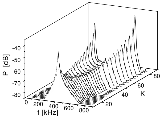
FIG. 9. Network analyser spectra of the control signal for the stabilised but disturbed orbit.
