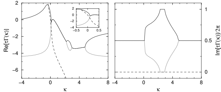
FIG. 7. Dependence of the exponents \tau\Gamma^{(1,2,3)}[\kappa] on real valued argument for the period-one orbit of the Rössler system for \varepsilon = 0 . \tau\Gamma^{(1)}[\kappa] (solid) connects to the free exponent \lambda^{(1)}\tau = 0.808 , \tau\Gamma^{(3)}[\kappa] (dotted) to \lambda^{(3)}\tau = -2.026 , and \tau\Gamma^{(2)}[\kappa] (dashed) to the Goldstone mode with \lambda^{(2)}\tau = 0 . The inset shows the bifurcation structure close to \kappa = 0 .
