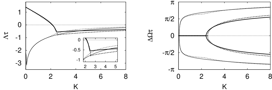
FIG. 5. Real part of two Floquet branches and frequency deviation for the period-one orbit of the Toda model (12) in dependence on the control amplitude (solid lines). Thick/thin line displays the branch connecting to the larger/smaller Lyapunov exponent of the free system. Dotted lines display results according to the analytical expressions (13) and (6). The inset shows an enlargement near to the control threshold.
