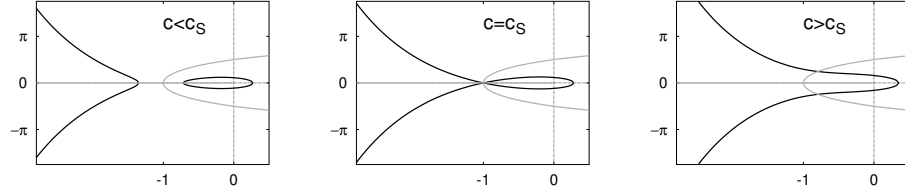
FIG. 14. Solution curves of eq.(B3) (solid lines) in the complex z plane for c < c_S , c = c_S , and c > c_S (from left to right). For comparison the solution of eq.(B4) is also shown (gray lines).
