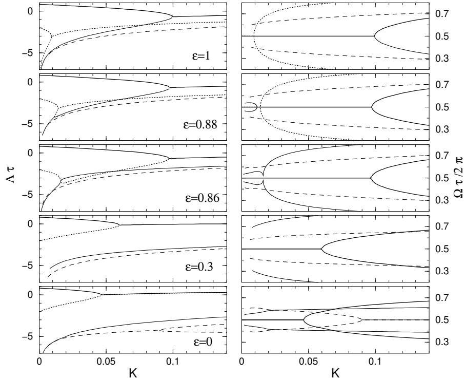
FIG. 6. Floquet exponents of the period-one orbit of the Rössler system (14) in dependence on the control amplitude. Thick solid/dotted line: branch originating from the free Lyapunov exponent \lambda^{(1)}\tau = 0.808 / \lambda^{(3)}\tau = -2.026 , dashed line: complex branch. The Goldstone mode connected to \lambda^{(2)}\tau = 0 is not displayed.
