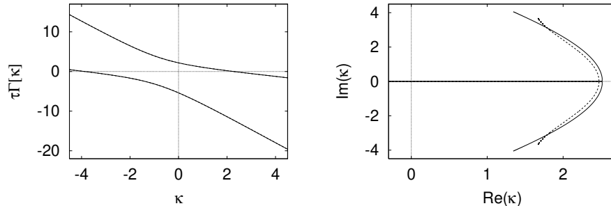
FIG. 4. Left: Dependence of the exponents \tau\Gamma^{(1,2)}[\kappa] on real valued argument. Right: Location of the Floquet exponents (cf. figure 3) in the complex \kappa plane (solid line). Dotted lines are results from the analytical expression (13), but coincidence is almost within the resolution of the figure.
