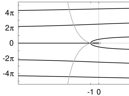
FIG. 15. Solution curves of eq.(B4) (solid lines) in the complex z plane. For comparison the solution of eq.(B3) for c = c_S is also shown (gray lines). The actual value of c does not essentially influence the large scale properties of the latter curve.
