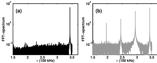
FIG. 3: Fourier spectrum of the measured signal at K = 9.76 and R = 0.12 for two different initial conditions: (a) controlled periodic orbit (adiabatic increase of the control amplitude), (b) delay induced quasiperiodic state (adiabatic decrease of the control amplitude).
