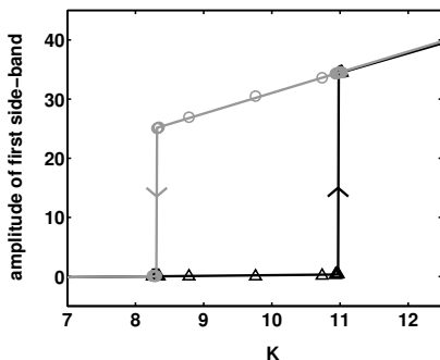
FIG. 4: Amplitude of the first side-band at 290 kHz vs. control amplitude K for R = 0.12 . Triangles: increasing K , circles: decreasing K . (cf. figure 3 for corresponding Fourier spectra).
