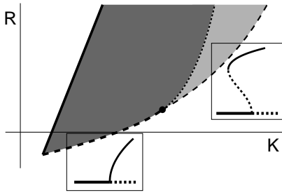
FIG. 1: Diagrammatic view of the control domain (dark and light grey-shaded) for extended time-delayed feedback control. Lower control threshold (solid line), upper control threshold (broken line), saddle node bifurcation of the delay induced orbit (dotted line). The dot indicates a transition from super- to subcritical behaviour (cf. insets for sketches of the bifurcation diagram). The corresponding region of bistability between the controlled orbit and the delay induced motion is light grey-shaded.
