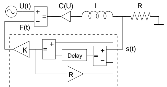
FIG. 2: Experimental setup of the nonlinear diode resonator with extended time-delayed feedback control device.
