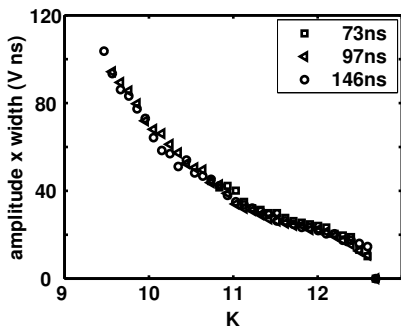
FIG. 6: Critical pulse strength in dependence on the control amplitude for different width of pulses and R = 0.12
