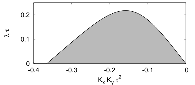
FIG. 1: Exact analytic result for the control domain of two \tau -periodic unstable orbits with Floquet exponents \mu = \nu = \lambda + i\pi/\tau , diagonal coupling, and time delays \theta = 2\tau , according to Eq.(3).
