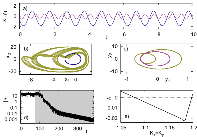
FIG. 2: (Color online) Numerical simulation of the Toda system, Eqs.(5). a) Time traces of the synchronised state for K_x = K_y = 1.15 (for other parameter values see the text). b,c) The motion in the phase plane of each oscillator without control (bronze) and with control (blue/red). d) Time dependence of the residual signal. The shaded region indicates the period where control K_x = K_y = 1.15 is applied. e) Dependence of the leading nontrivial Lyapunov exponent on the control gain as estimated from the exponential decay of the residual control signal (the two vanishing Lyapunov exponents are not displayed).
